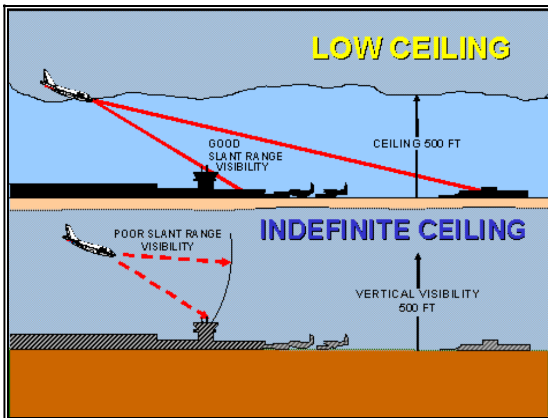
Figure 3-3. Obscuration Effects on Slant Range Visibility The ceiling is 500 feet in both examples, but the indefinite ceiling example (bottom) produces a more adverse impact to landing aircraft. This is because an obscuration (e.g., fog, blowing dust, snow, etc.) limits runway
